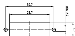
Panel cutout
