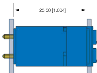
Straight PCB Mount (Male) to Panel Mount Crimp (Female)
