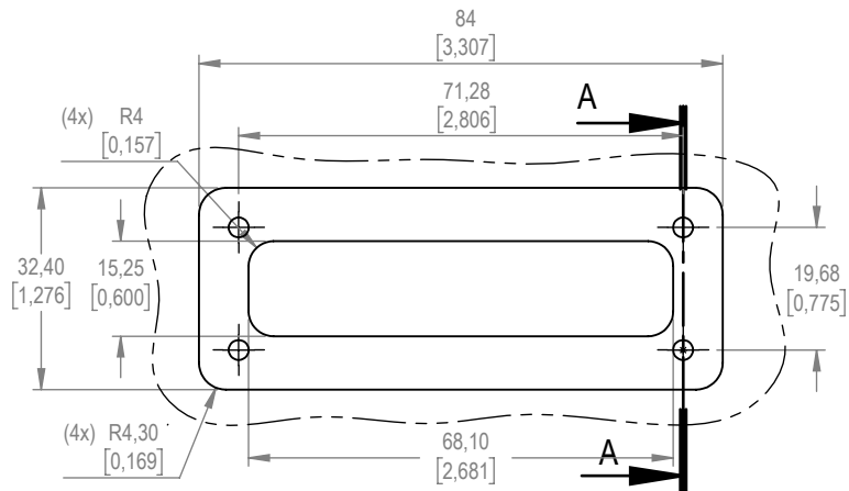
PANEL CUT-OUT INFORMATION
